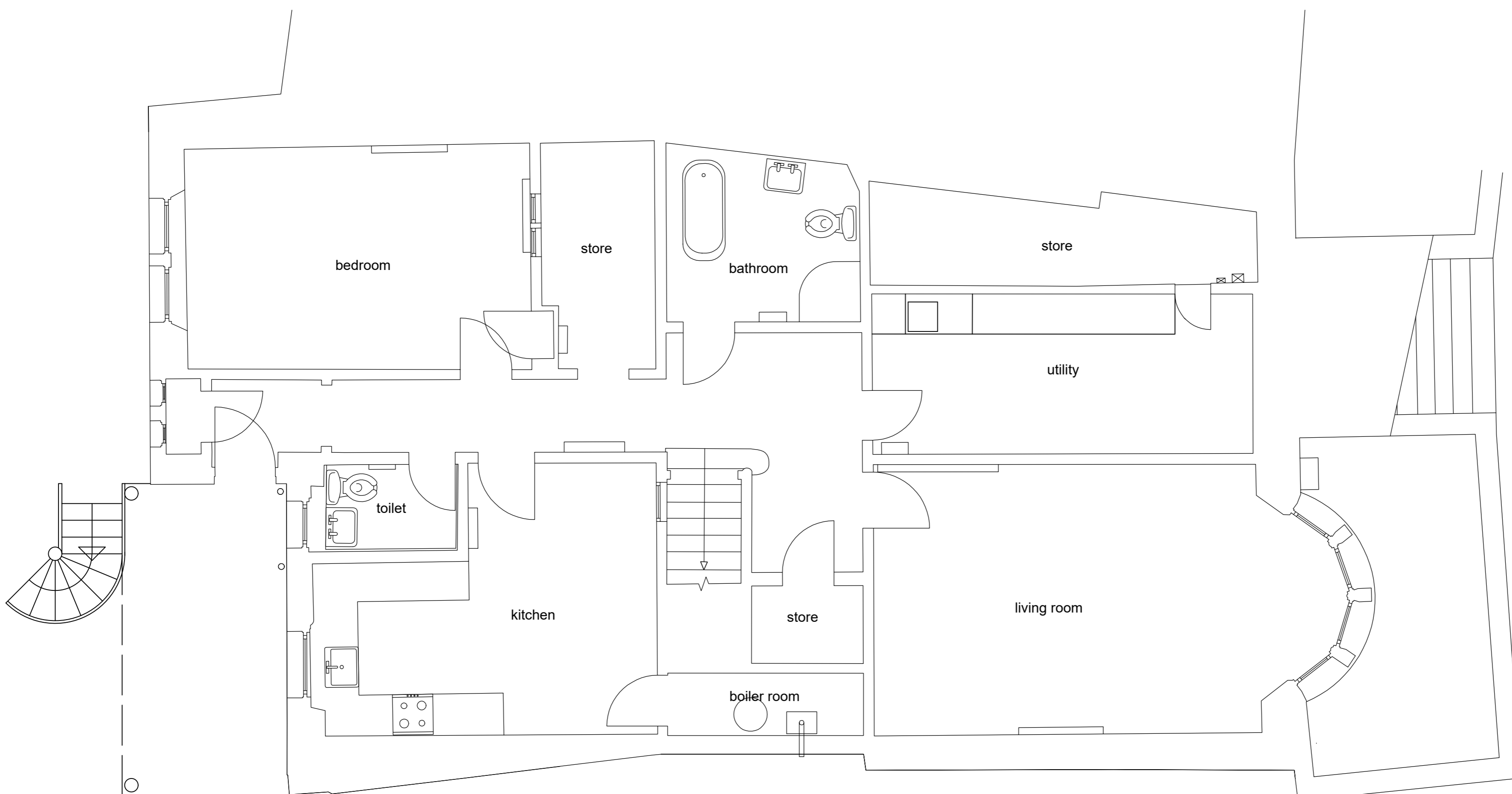
lower ground floor as proposed
