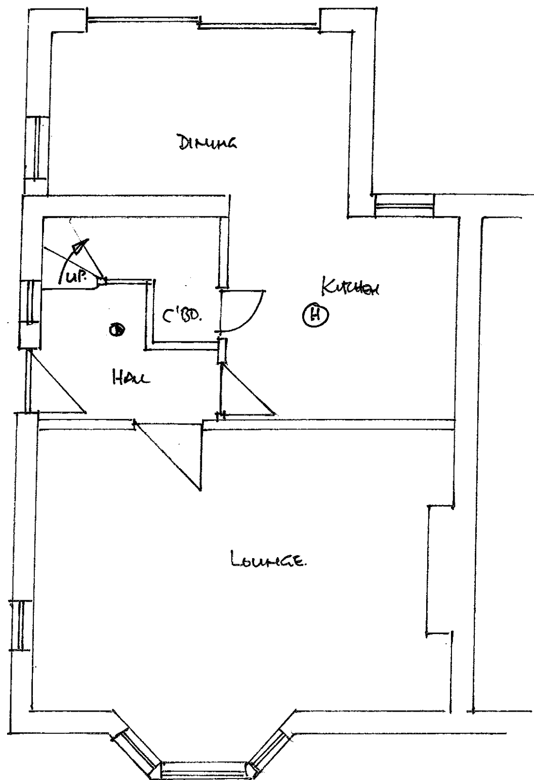
EXISTING Ground Floor Plan 1:50 @ A3
