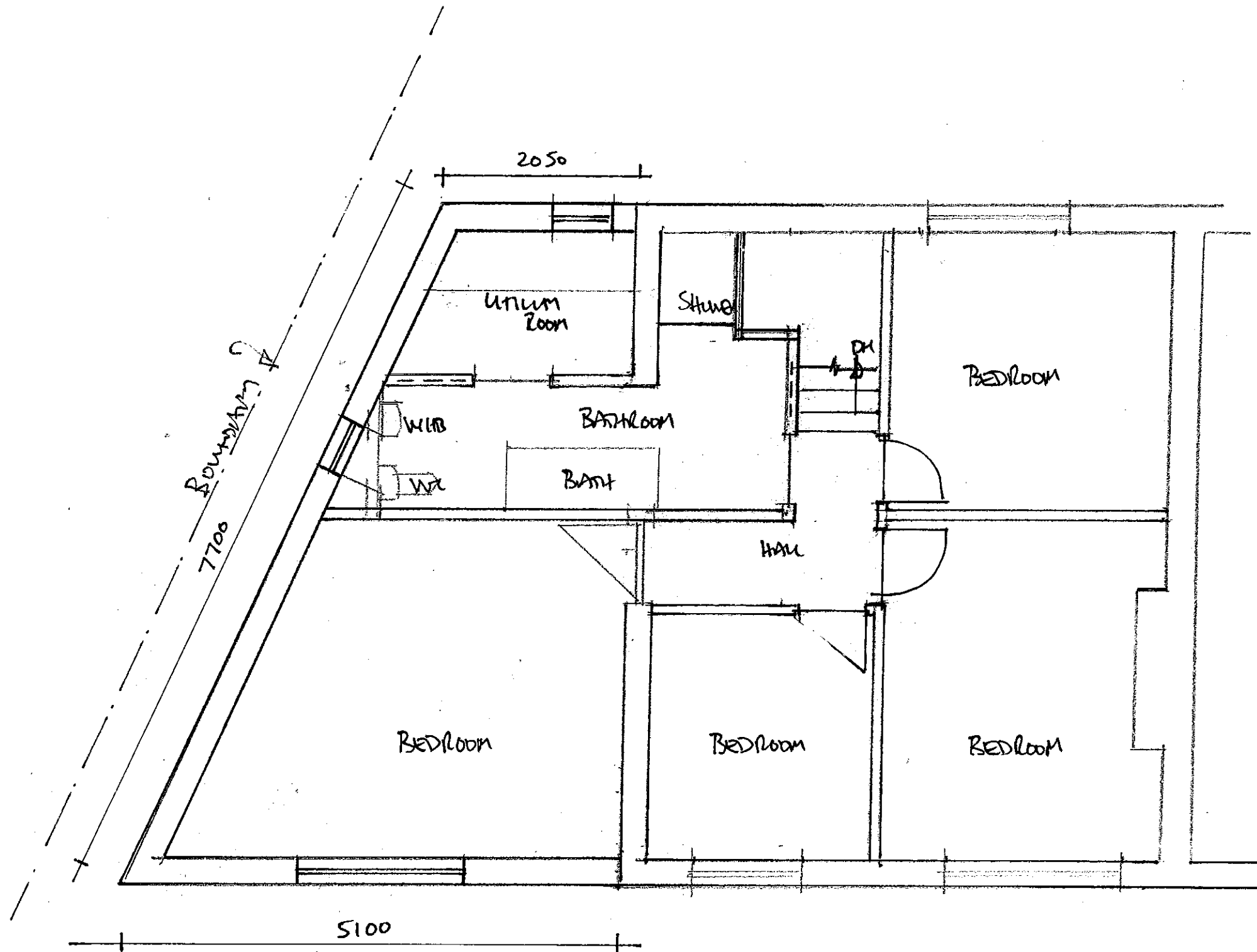
PROPOSED UPPER FLOOR PLAN 1:50 @ A3
