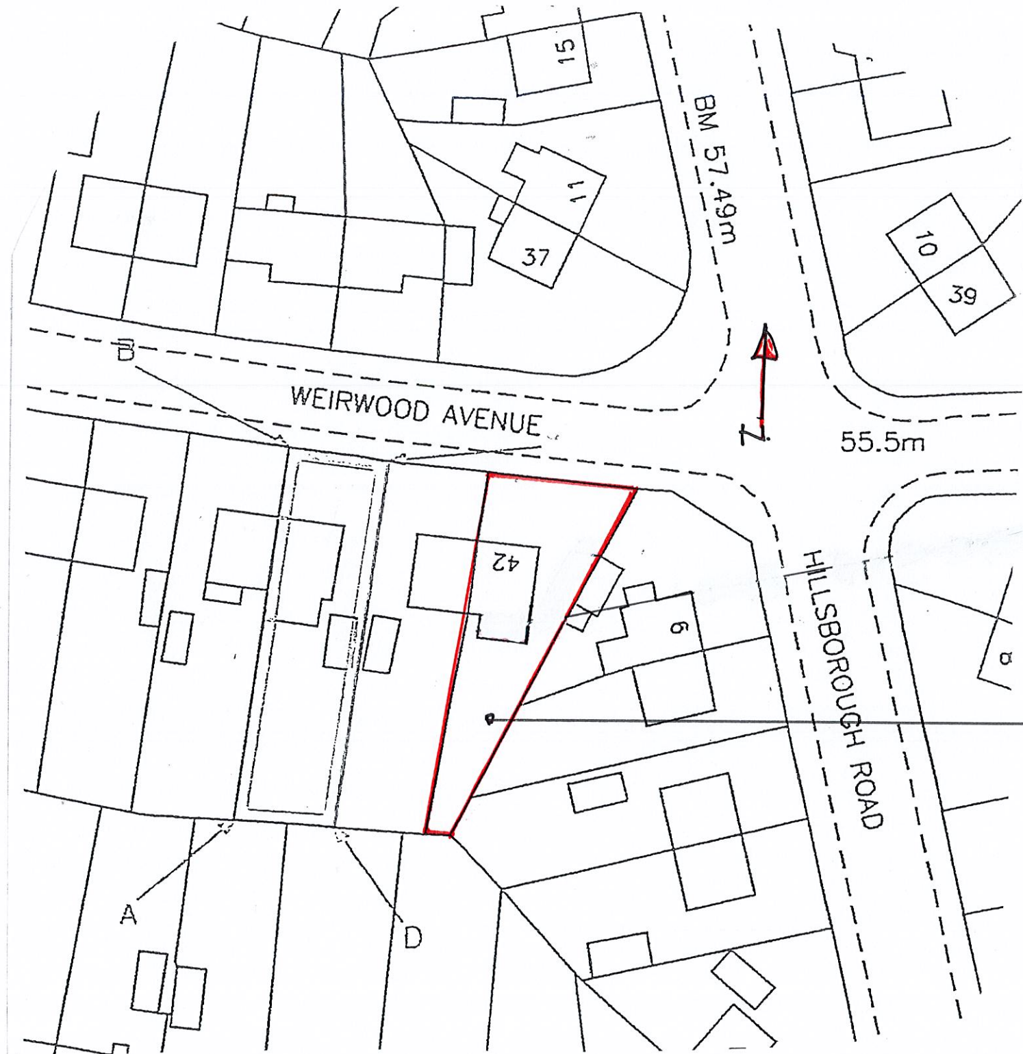
EXISTING BLOCK PLAN 1:500 @ A3
