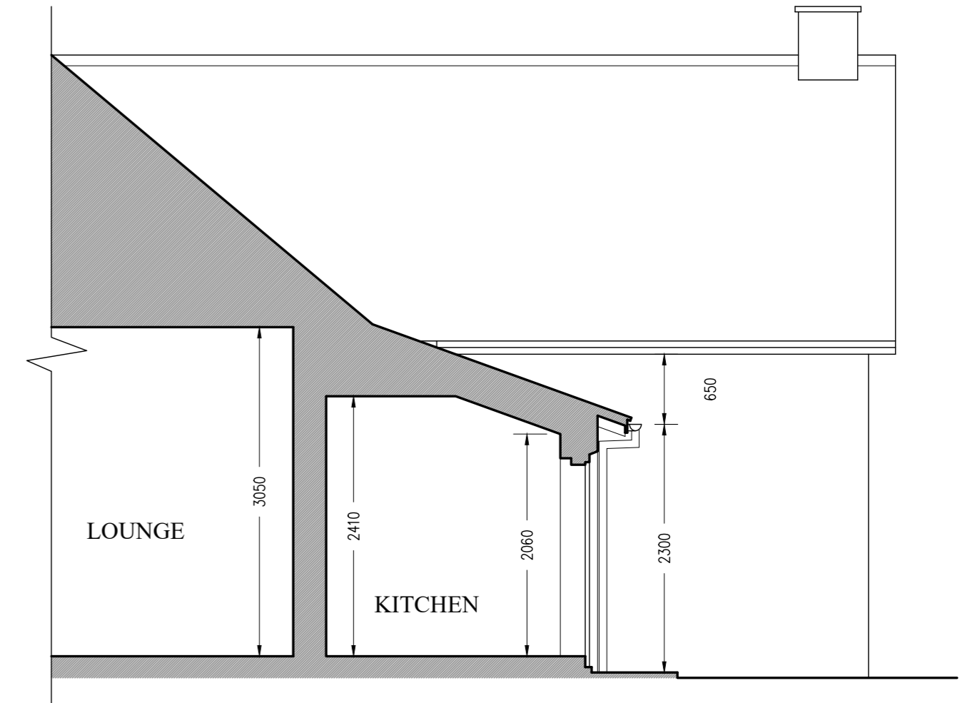
SECTION B-B
