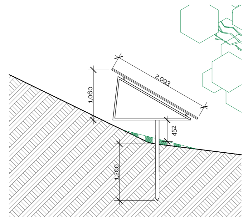
Section BB Solar Panels 1:50
