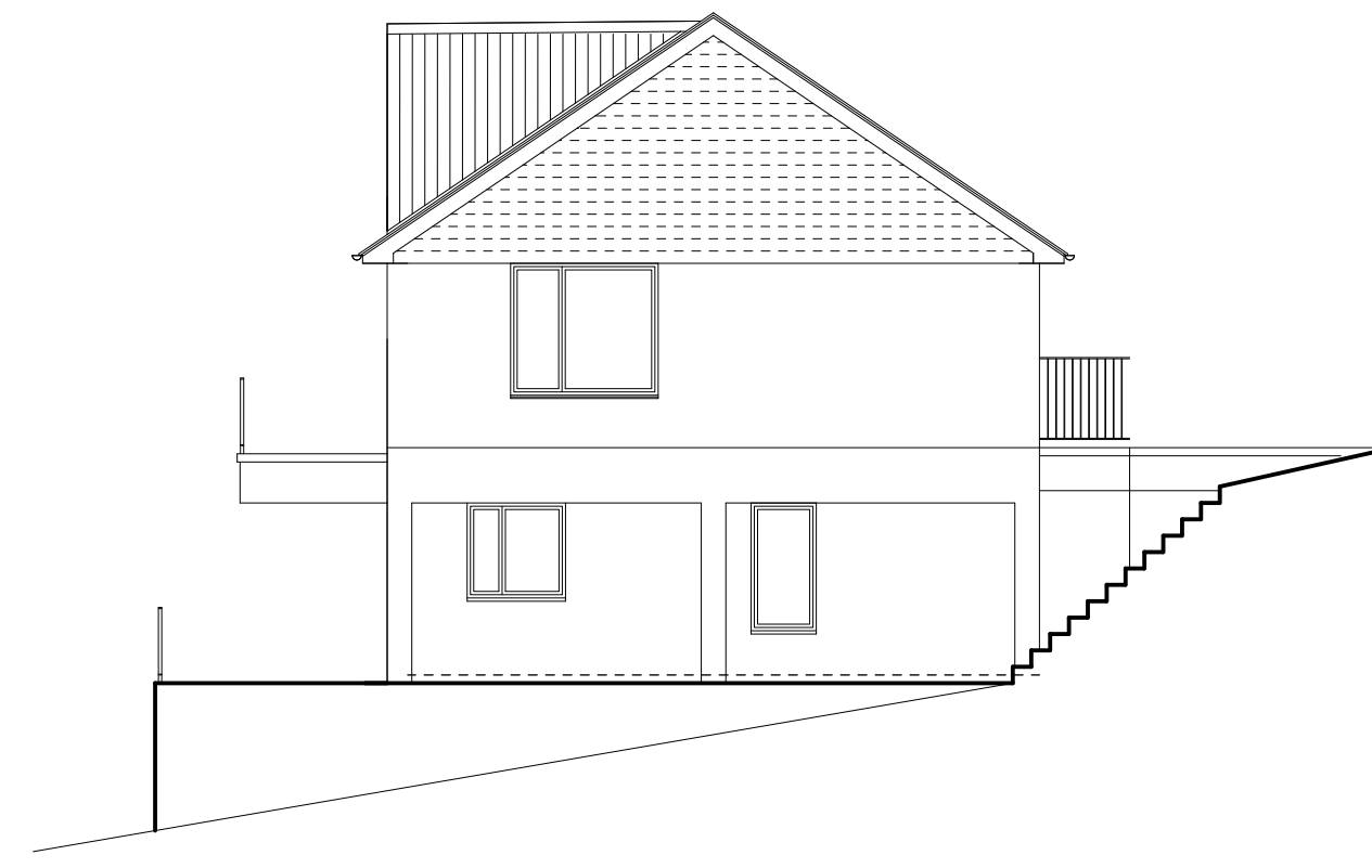
North Elevation
