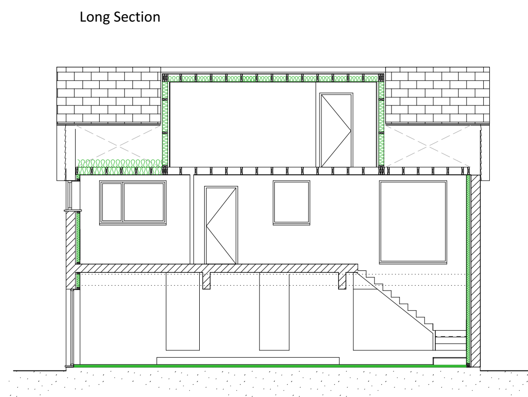
Long Section
