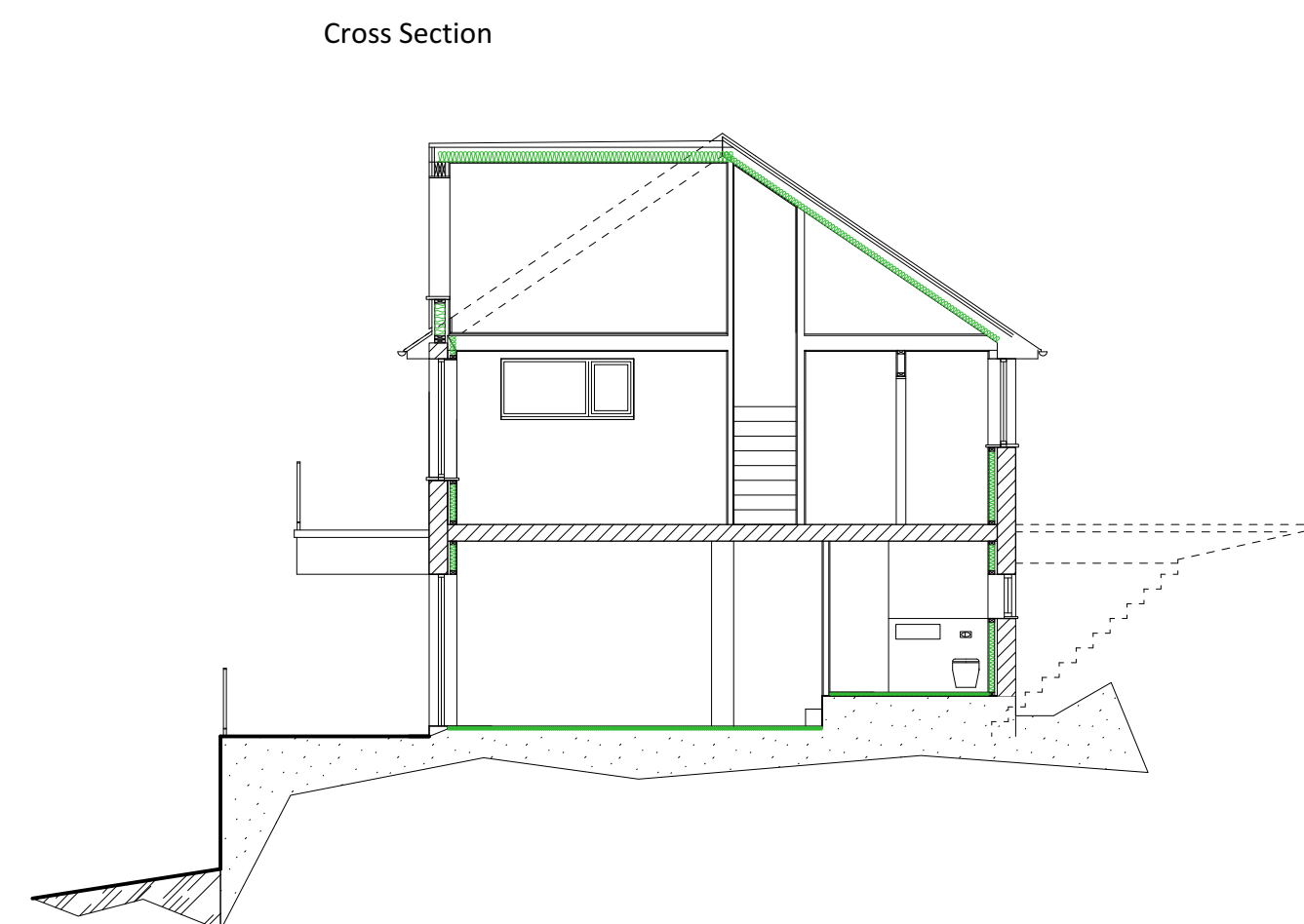
Cross Section
