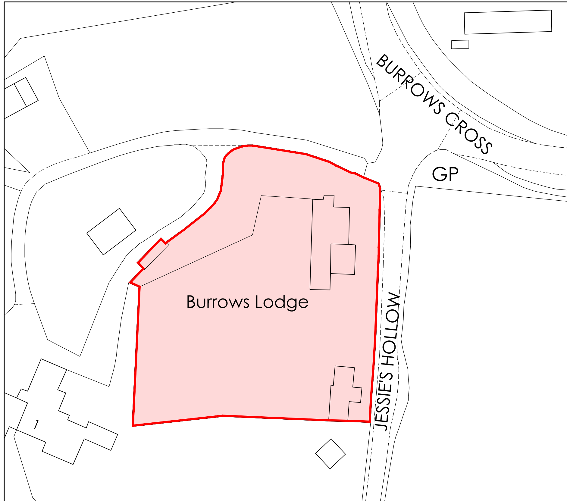
Block Plan
