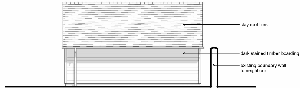
NORTH-WEST ELEVATION
