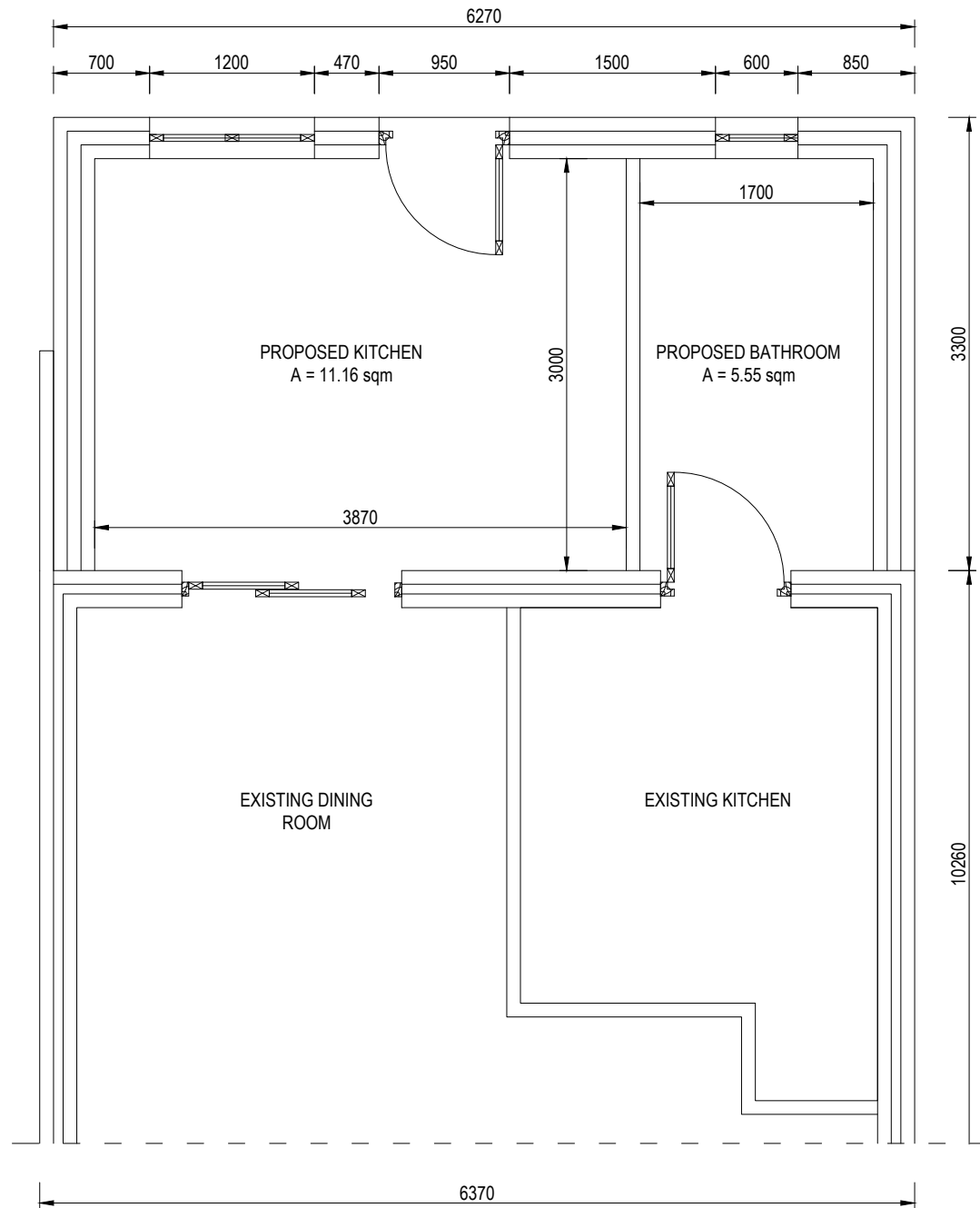
GROUND FLOOR EXTENSION PLAN
