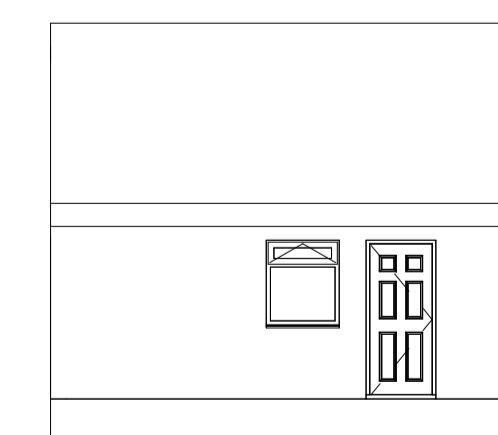
Garage Side Elevation - West 1 : 100
