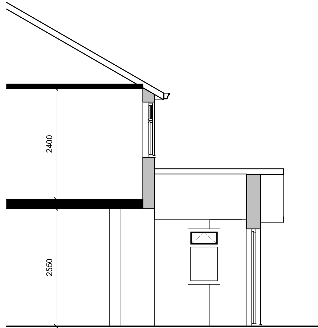
Proposed Section 1 1 : 50
