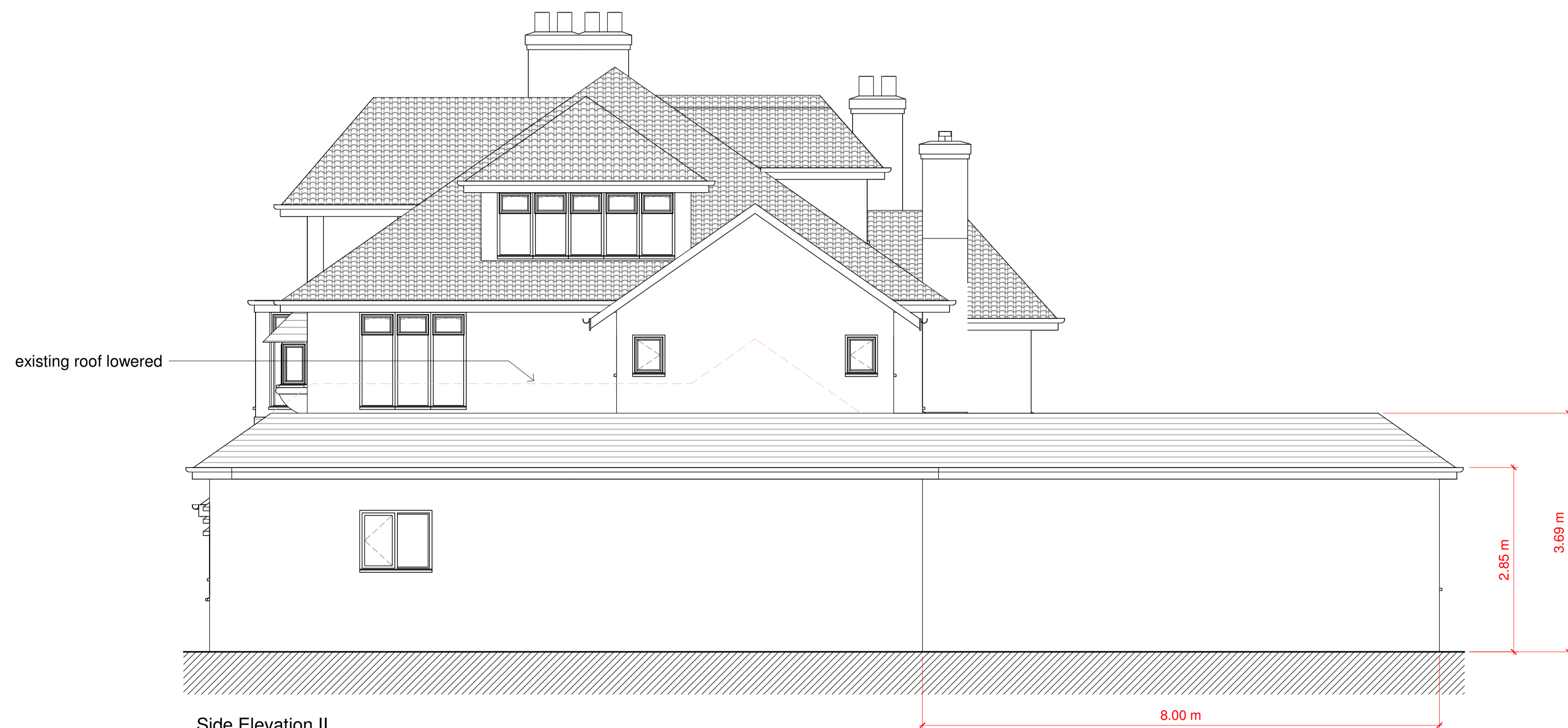
Side Elevation II. 1:50
