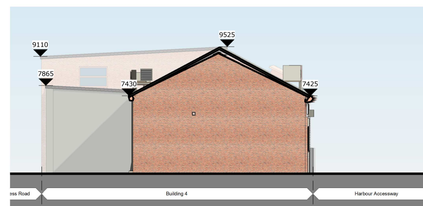
B4 - Existing Side Elevation (South East) SCALE: 1 : 100
