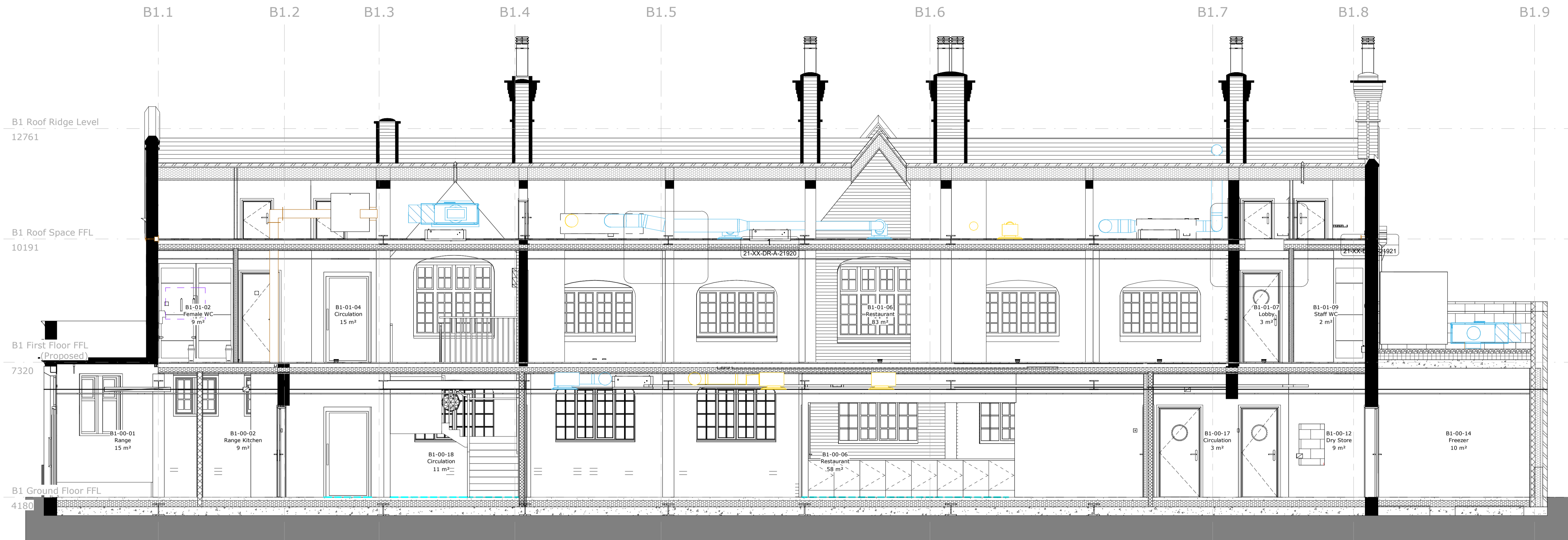
1 Building 1 - Proposed Detailed Arrangement Section A-A SCALE: 1 : 50
