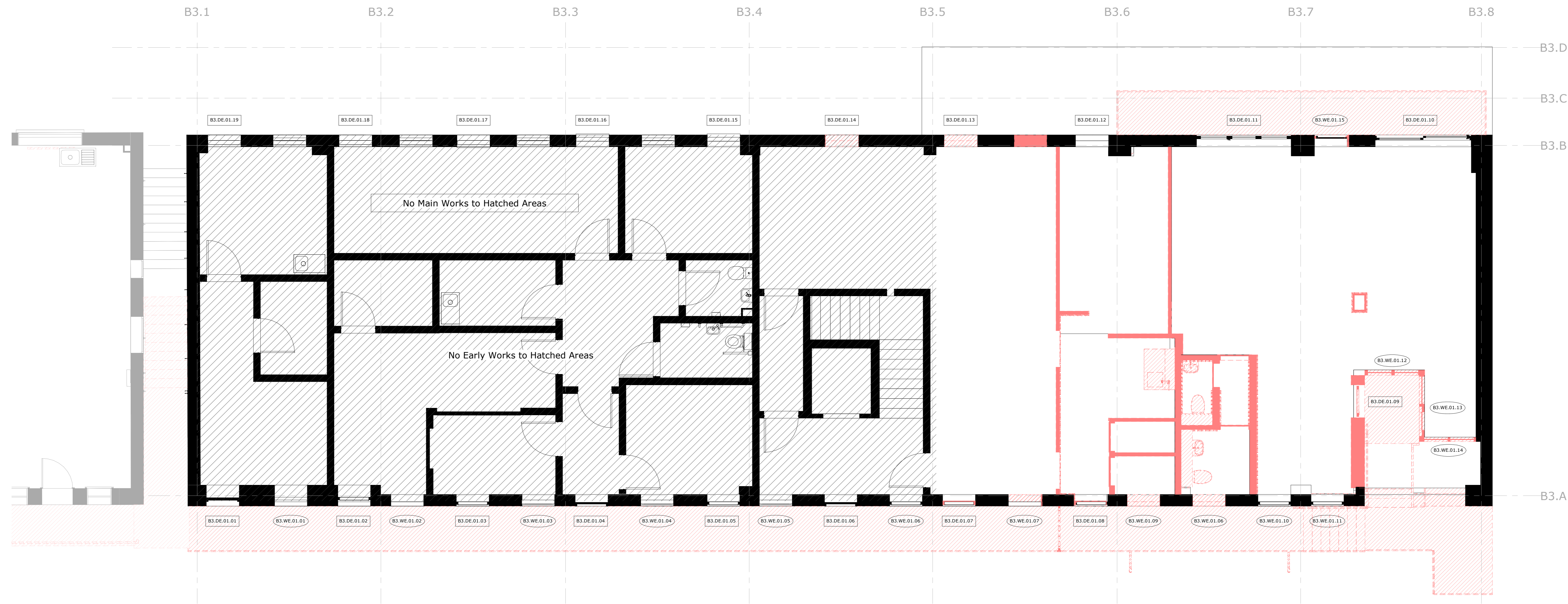
Building 3 - Main Works Proposed First Floor Demolition Plan SCALE: 1 : 50
