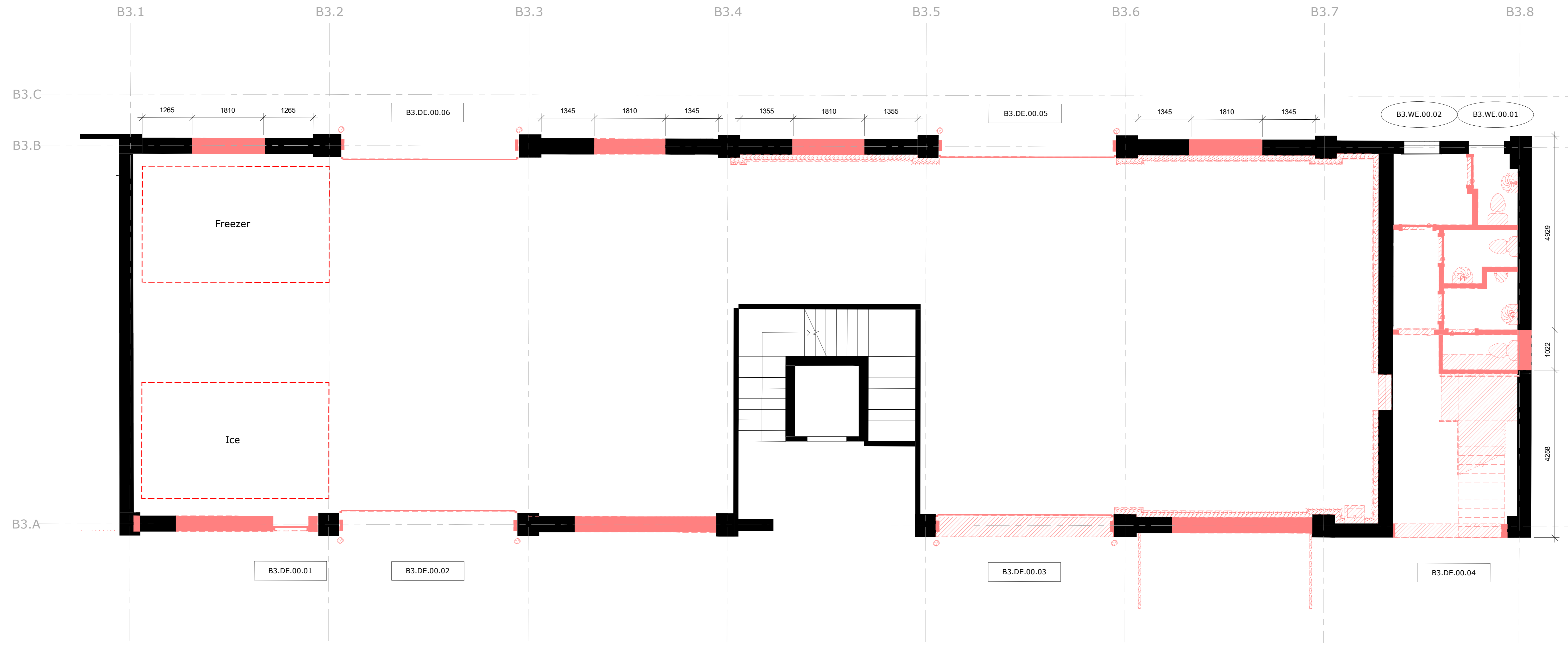
Building 3 - Main Works Proposed Ground Floor Demolition Plan SCALE: 1 : 50
