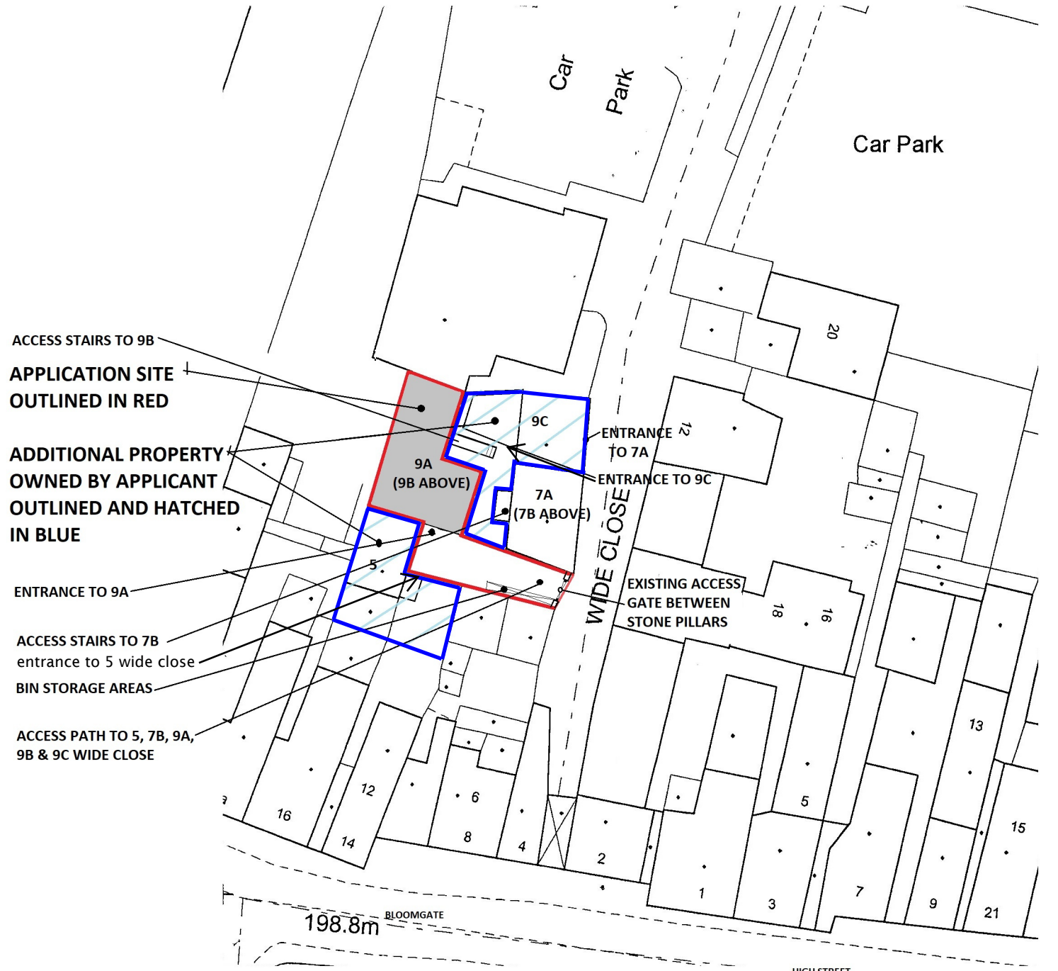
EXISTING/PROPOSED BLOCK PLAN SCALE 1:500
