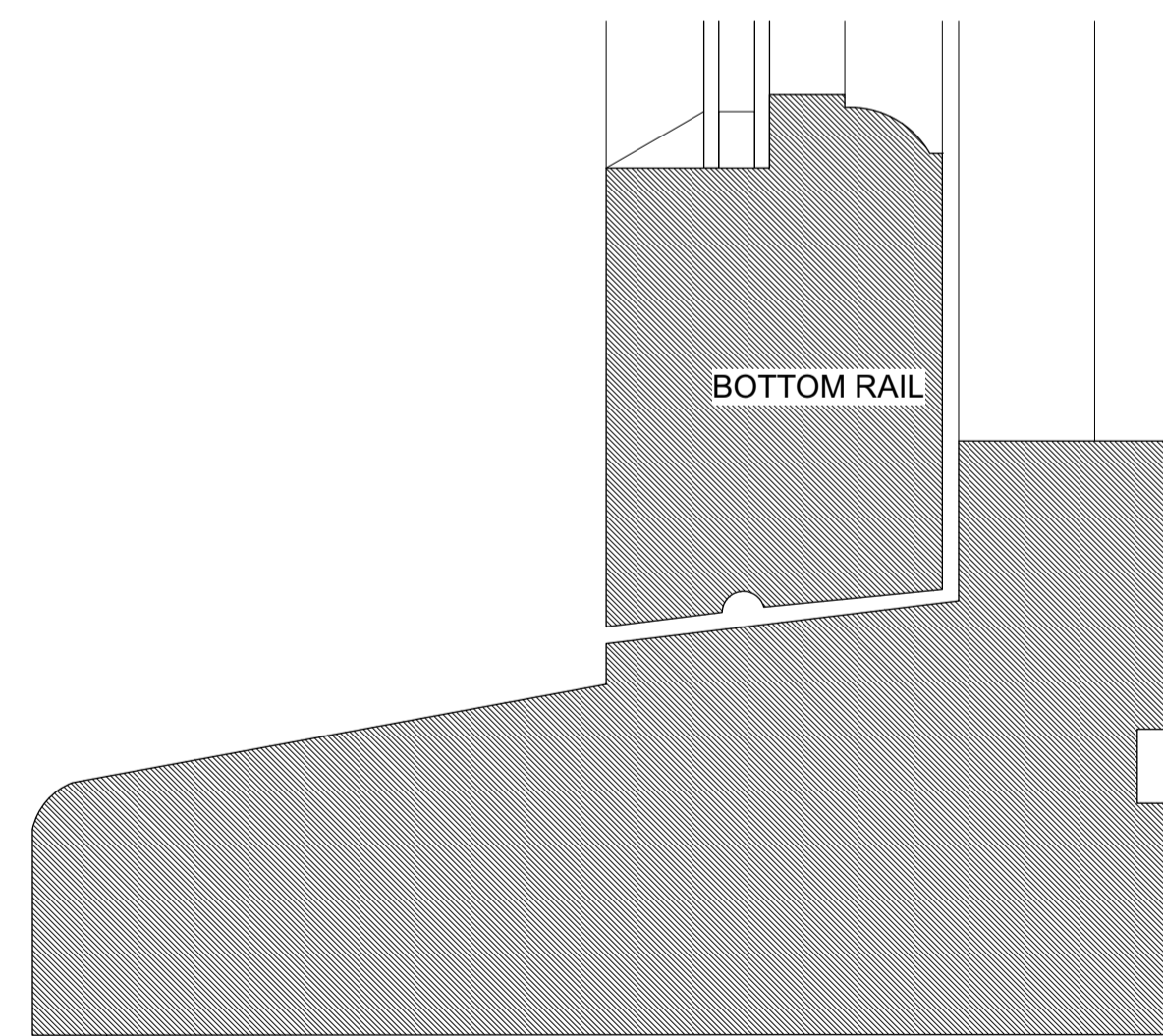
PROPOSED VERTICAL CROSS SECTION OF PROPOSED CASEMENT WINDOW
