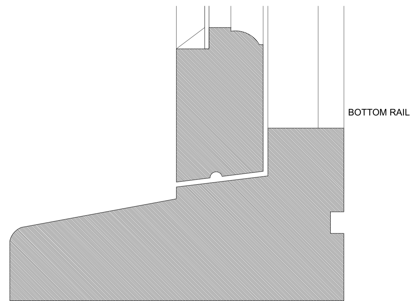
EXISTING VERTICAL CROSS SECTION OF EXISTING CASEMENT WINDOW
