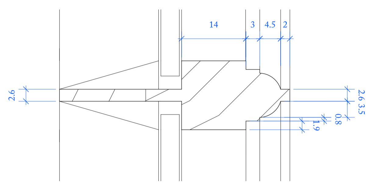
3 HISTORIC GLAZING BAR 1:1 @ A3
