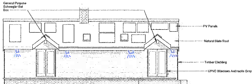
Front Elevation
