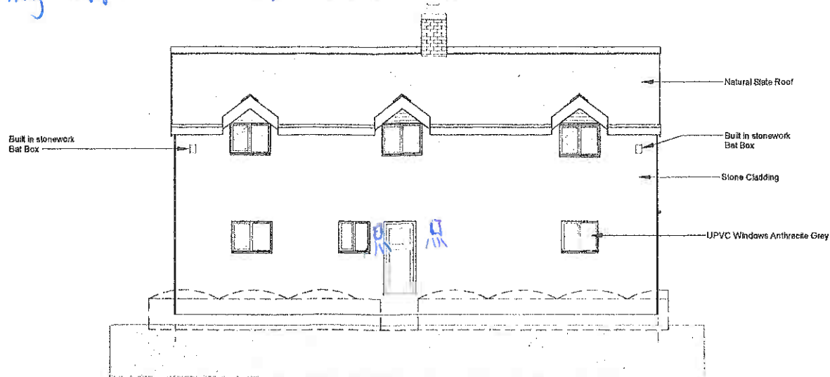
Front Elevation
