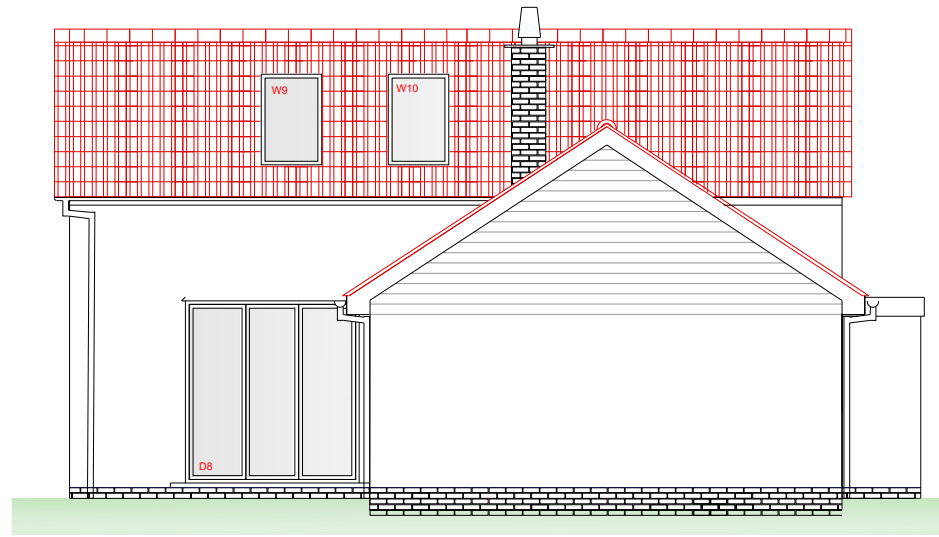
West Elevation 1:100
