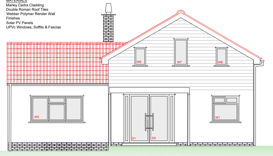
South Elevation 1:100
