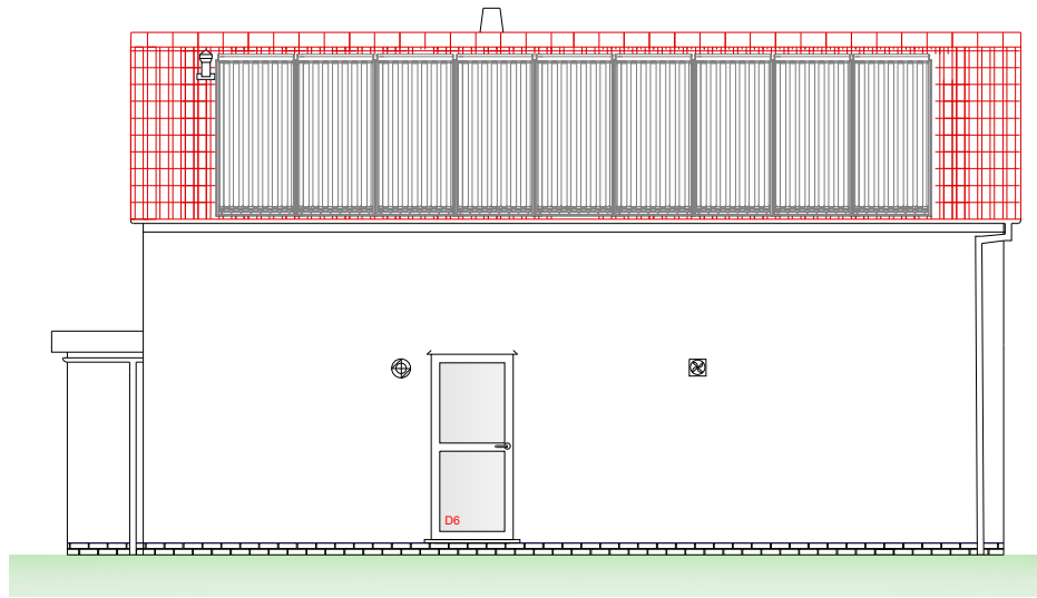
East Elevation 1:100
