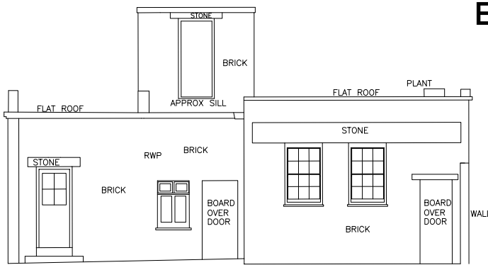
EXISTING FRONT DOOR ELEVATION
