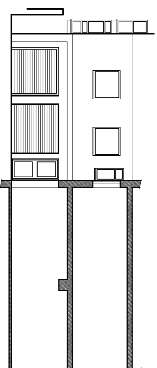
East Elevation (2-2) As Existing 1:100
