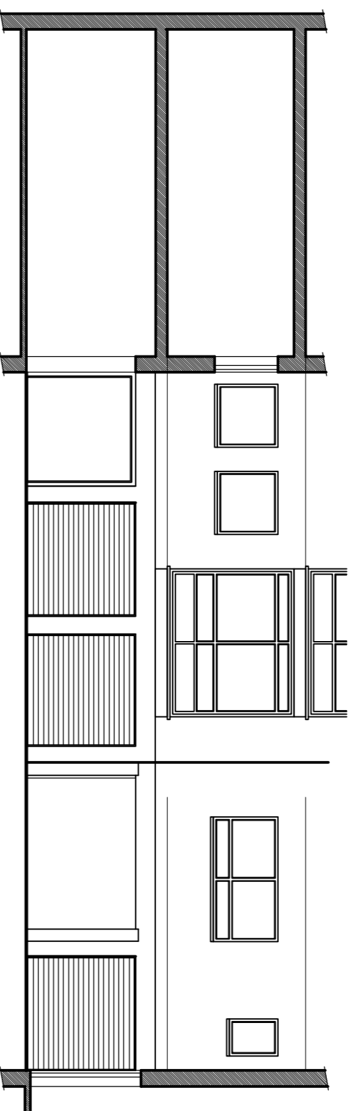
South Elevation (1-1) As Existing 1:100
