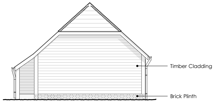
North Elevation Proposed
