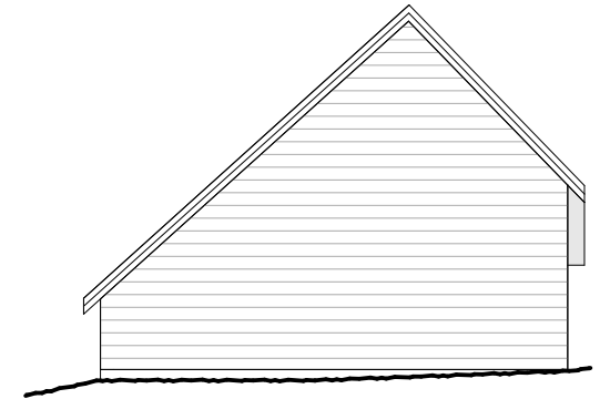
West Elevation
