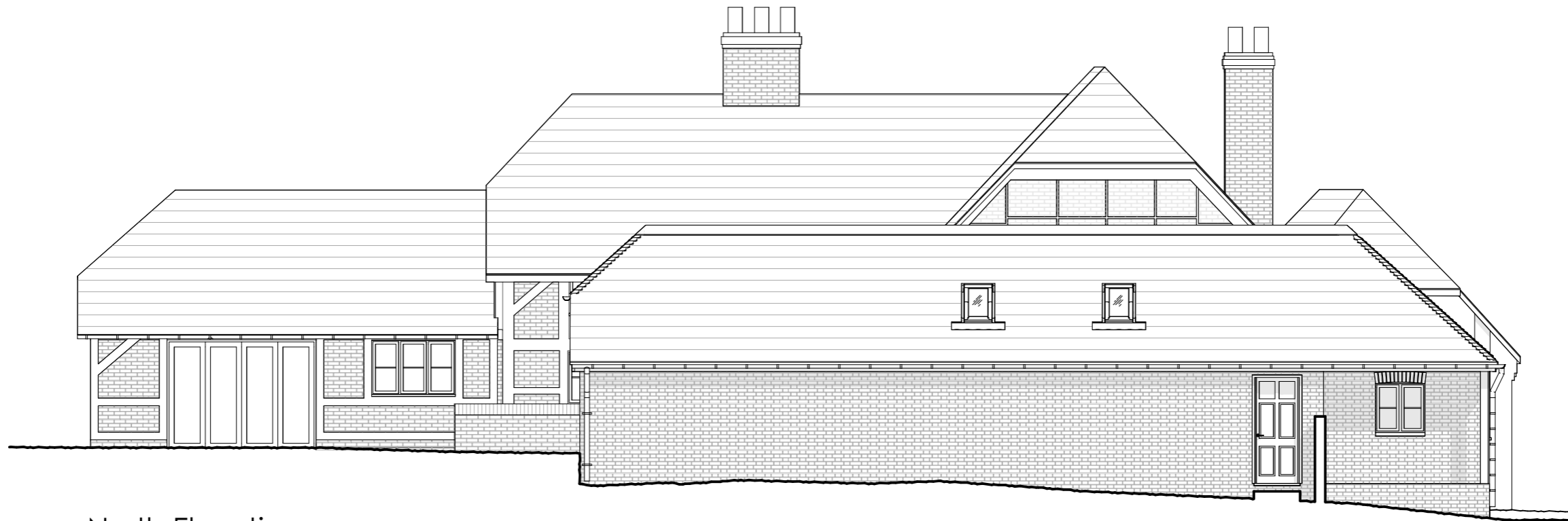
North Elevation
