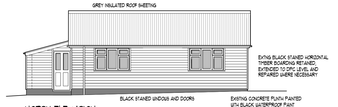
NORTH ELEVATION
