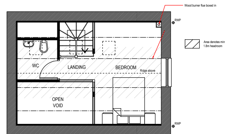
MEZZANINE LEVEL FLOOR PLAN
