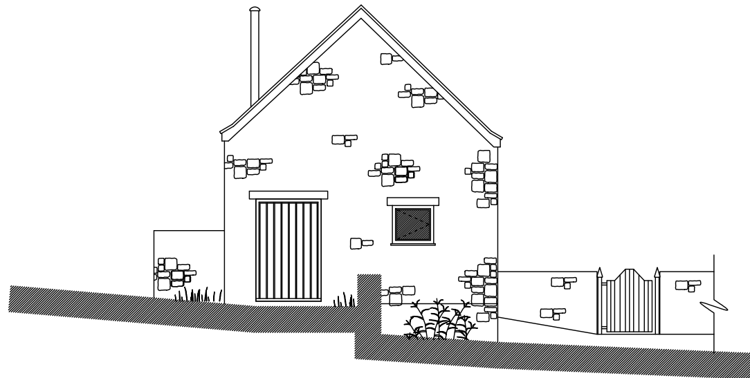
REAR ELEVATION WEST
