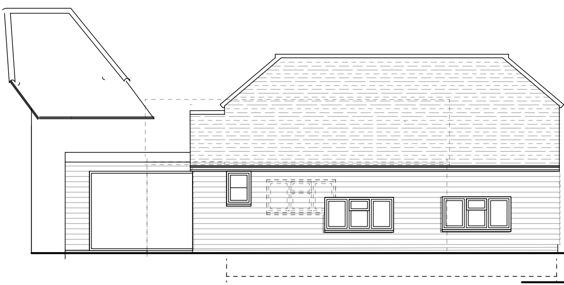
WEST ELEVATION
