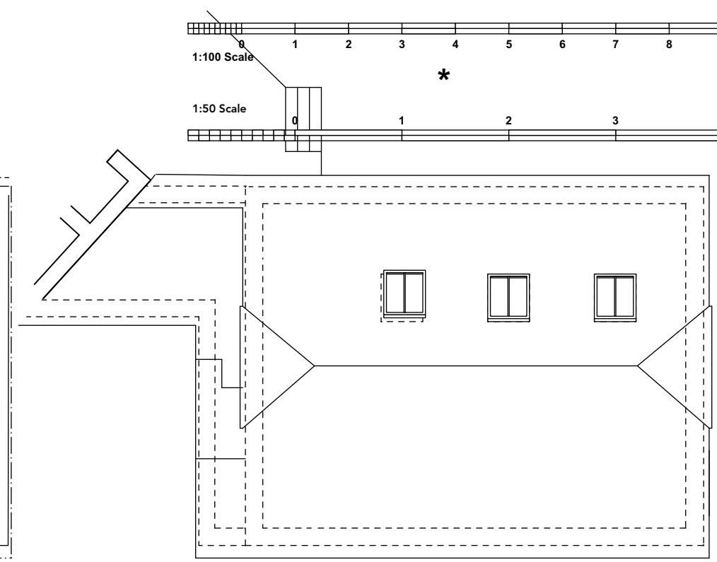
ROOF PLAN
