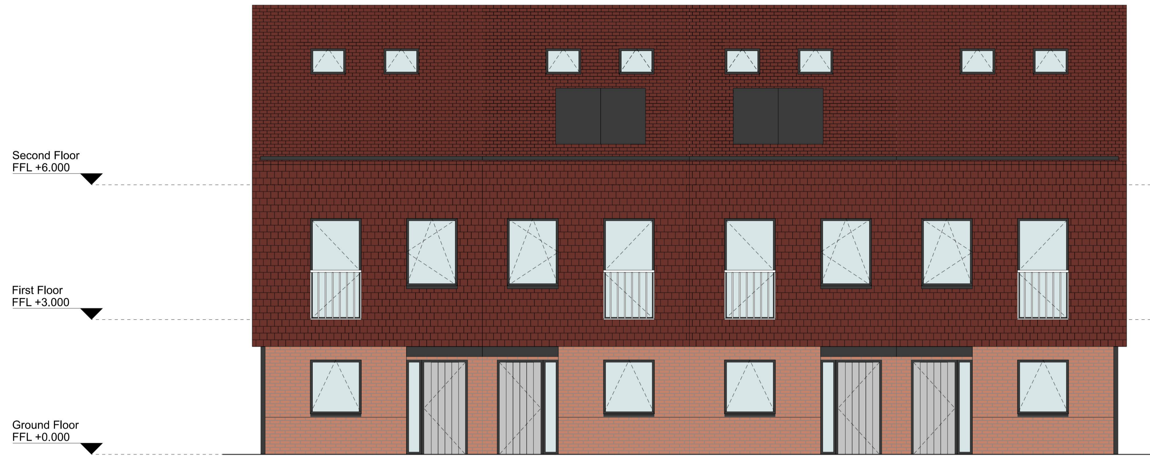
01 Terrace Front Elevation 04-0002 SCALE 1:50
