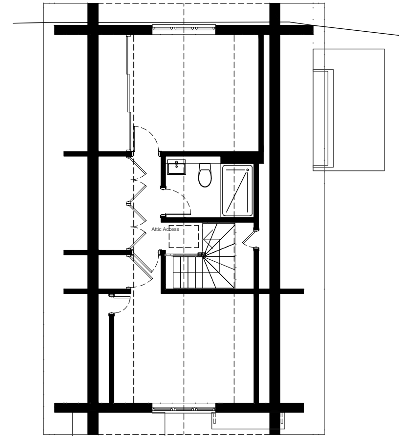
existing second floor plan 1:100
