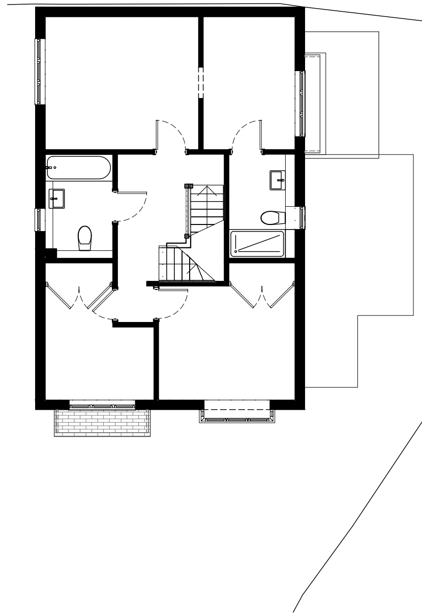
existing second floor plan 1:100
