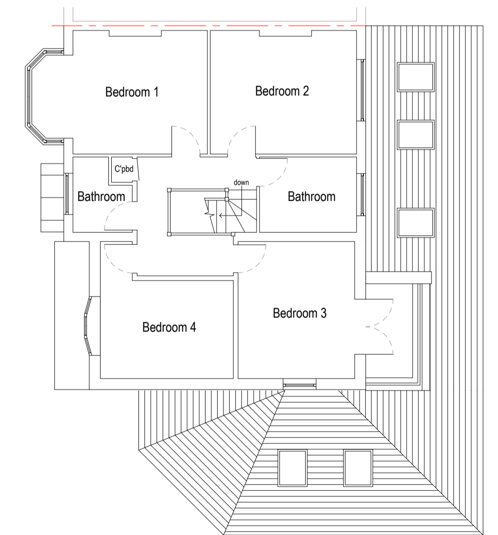
First Floor Proposed
