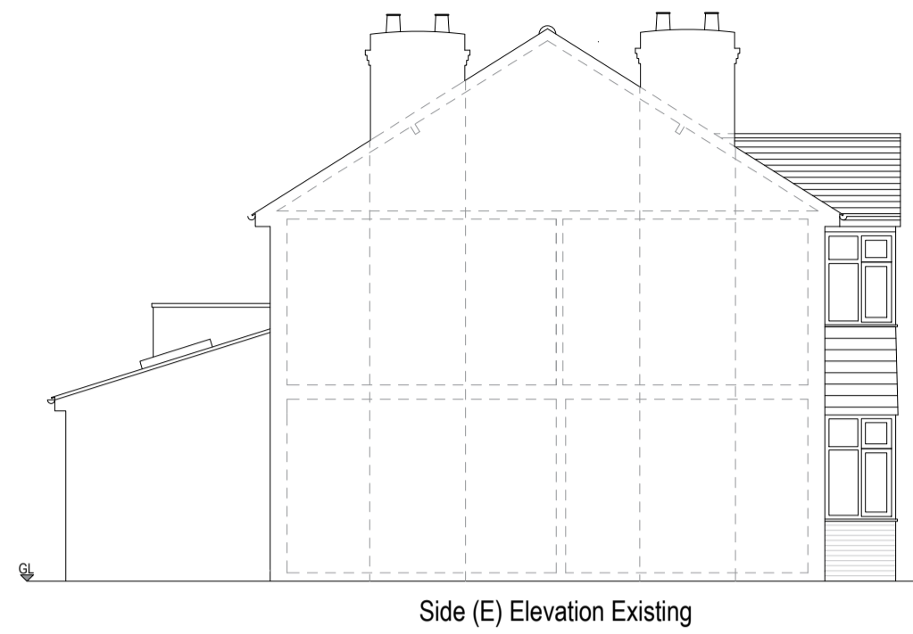
Side (E) Elevation Existing
