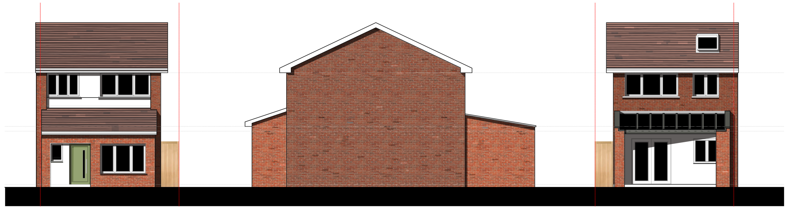
FRONT ELEVATION_PROPOSED
