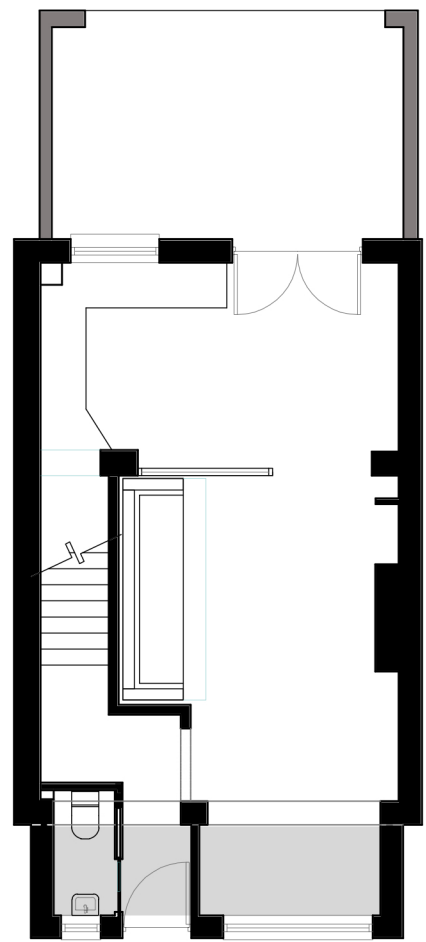
GROUND FLOOR_PROPOSED
