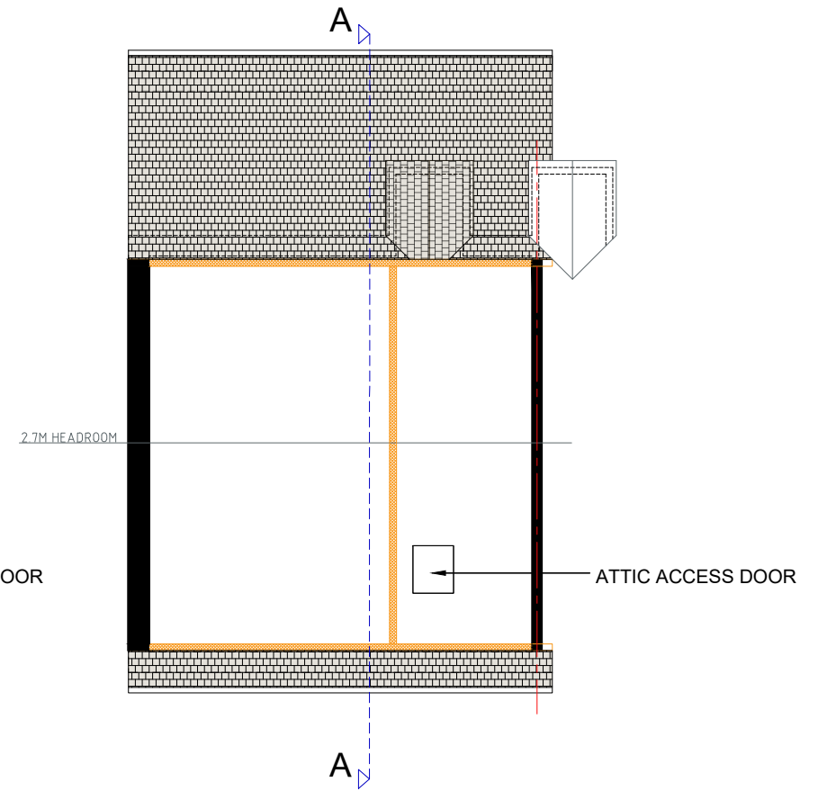
ATTIC PLAN Sc.1:100
