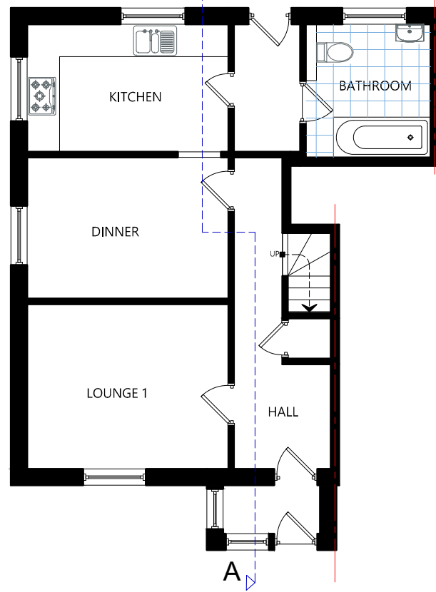
GROUND FLOOR PLAN Sc.1:100
