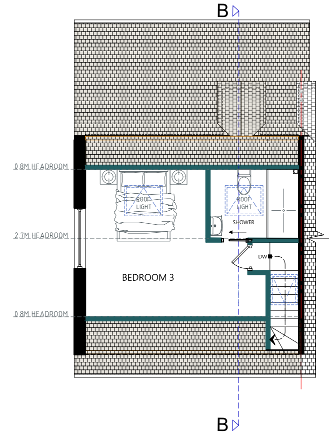
ATTIC PLAN Sc.1:100
