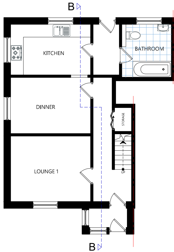
GROUND FLOOR PLAN Sc.1:100
