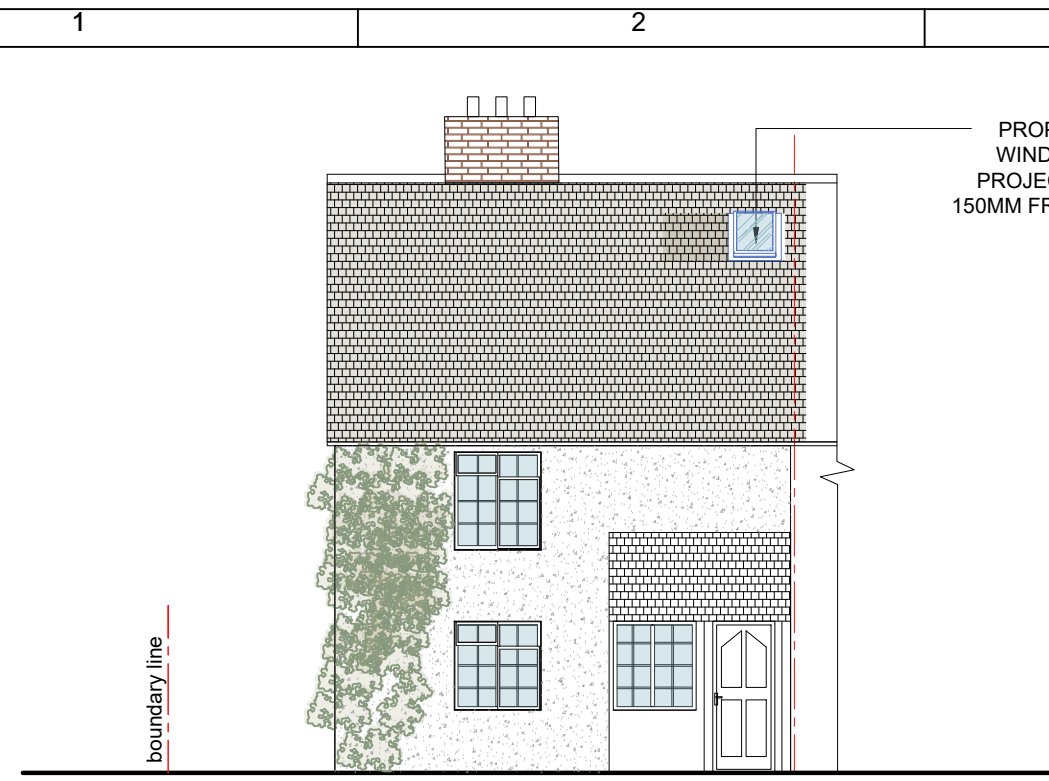
FRONT ELEVATION (SOUTH) Sc.1:100
