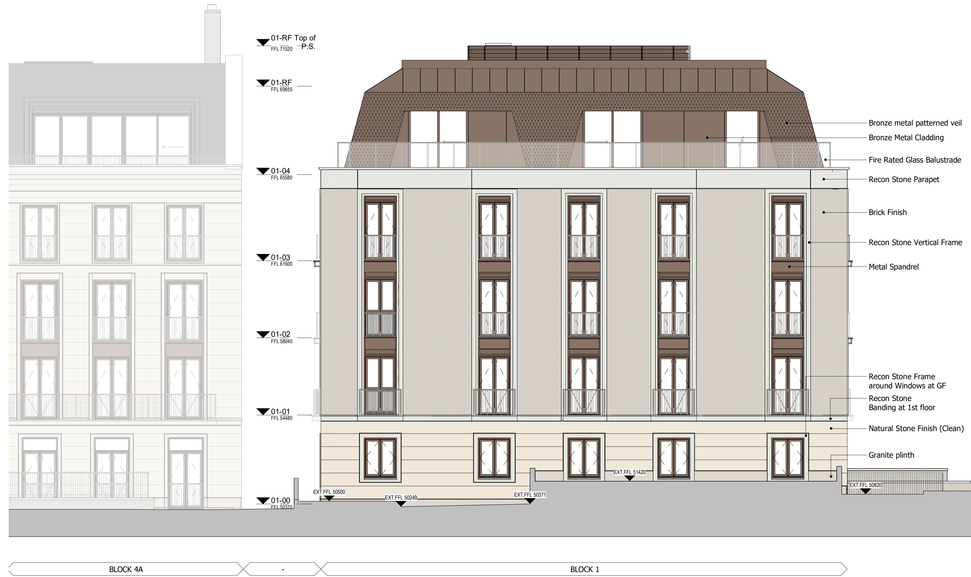
1 Block 1 - North West Elevation 1:100
