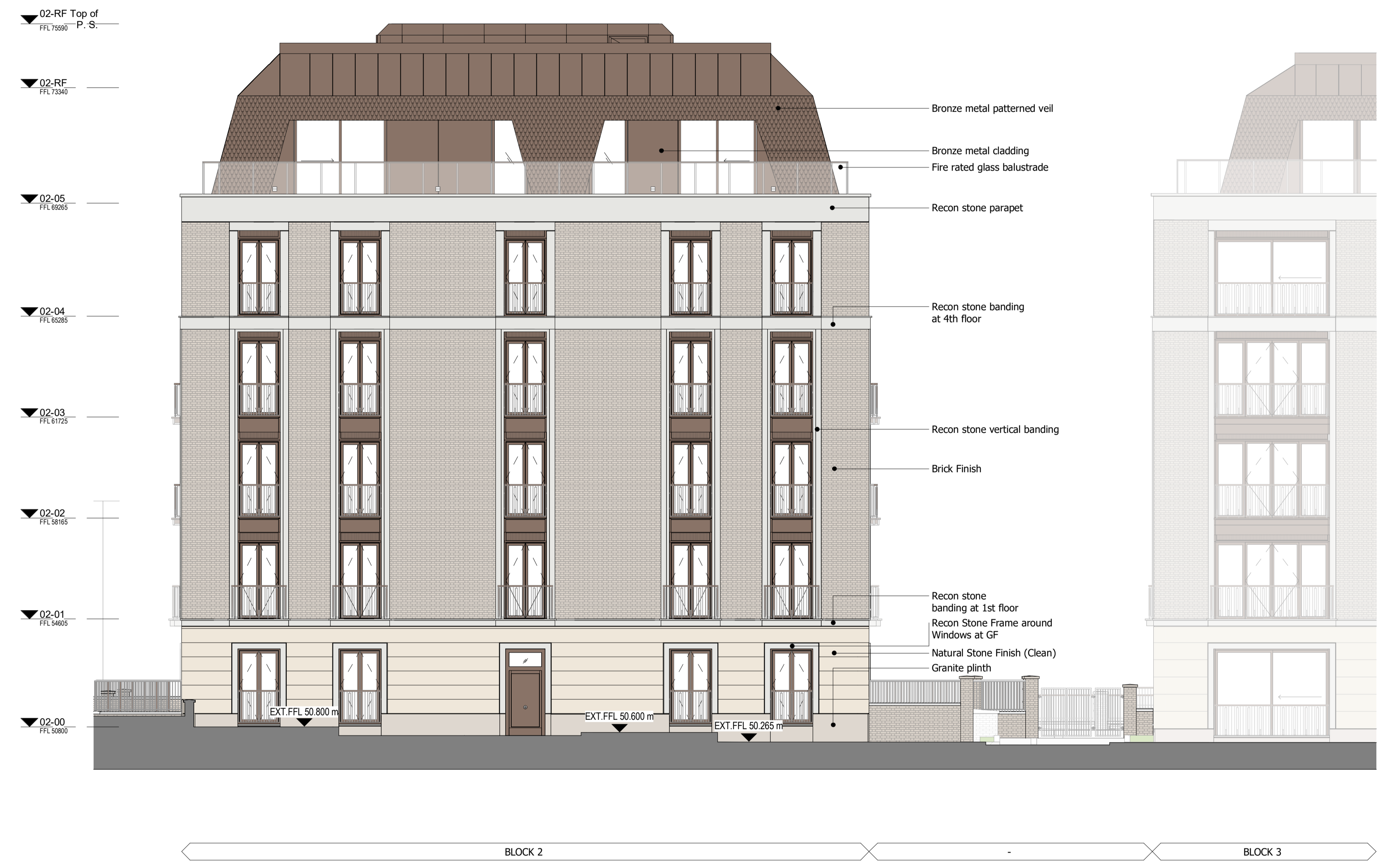
1 Block 2 - South East Elevation 1 : 100
