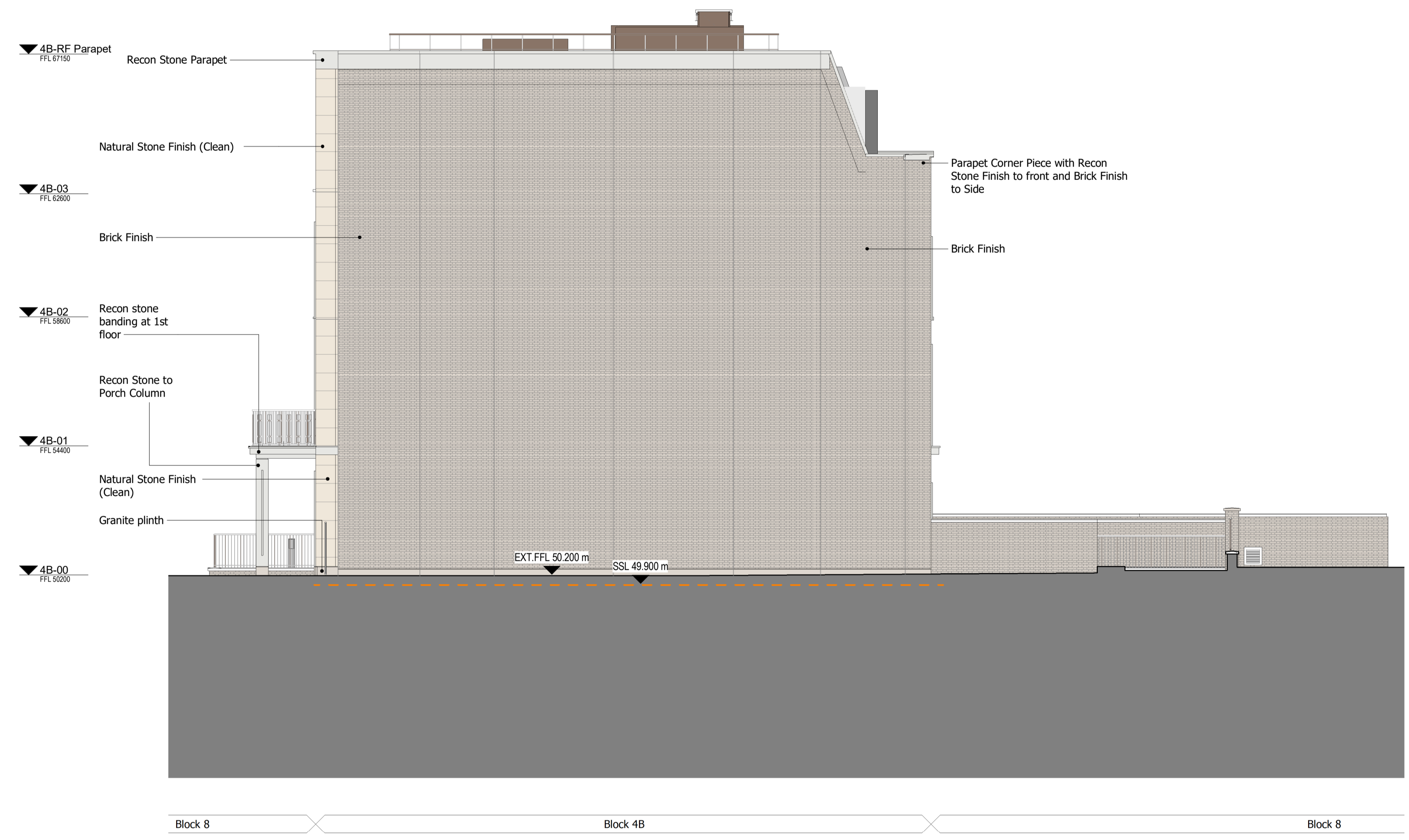
1 South West Elevation Finishes 1:100
