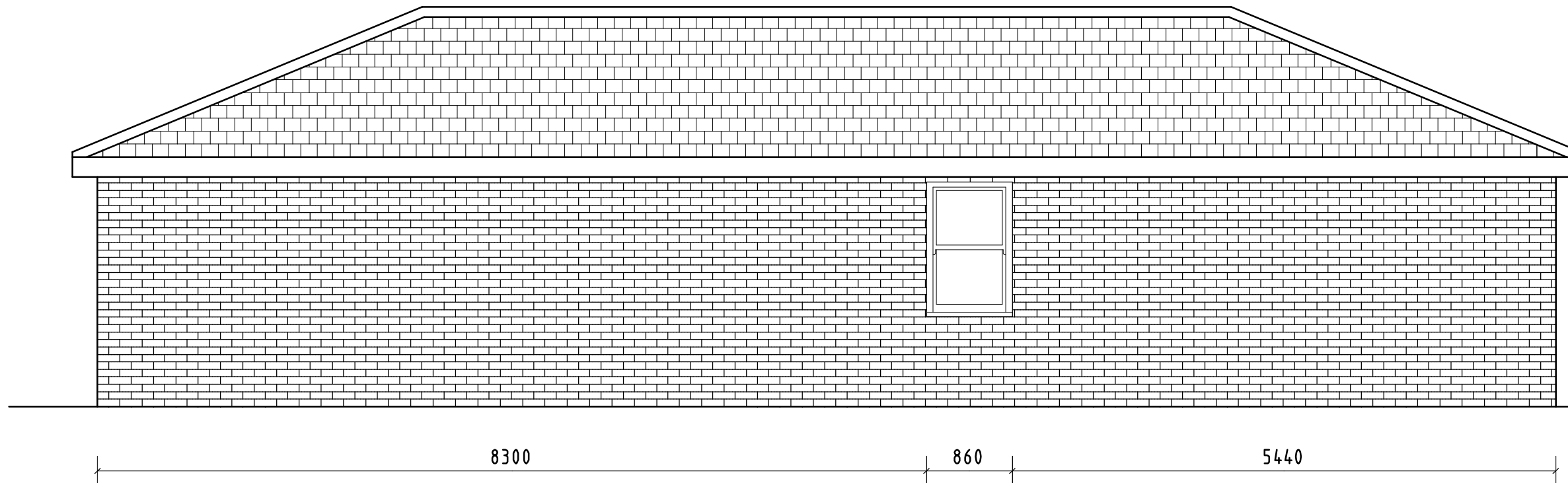
Existing and Proposed West Elevation
