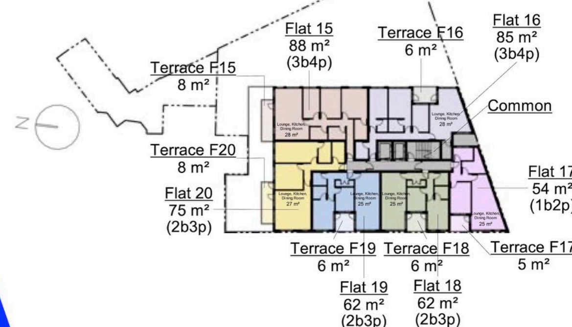
2 Third Floor Area Plan 1 : 500
