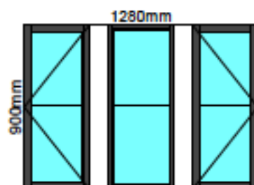
Window - (W4) Front - Ground Floor
