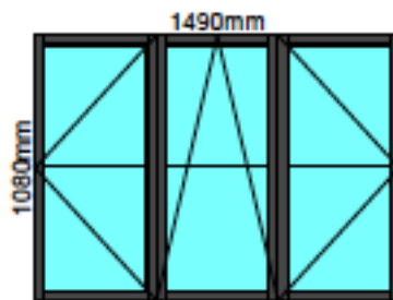
Window - (W2) Front - First Floor
