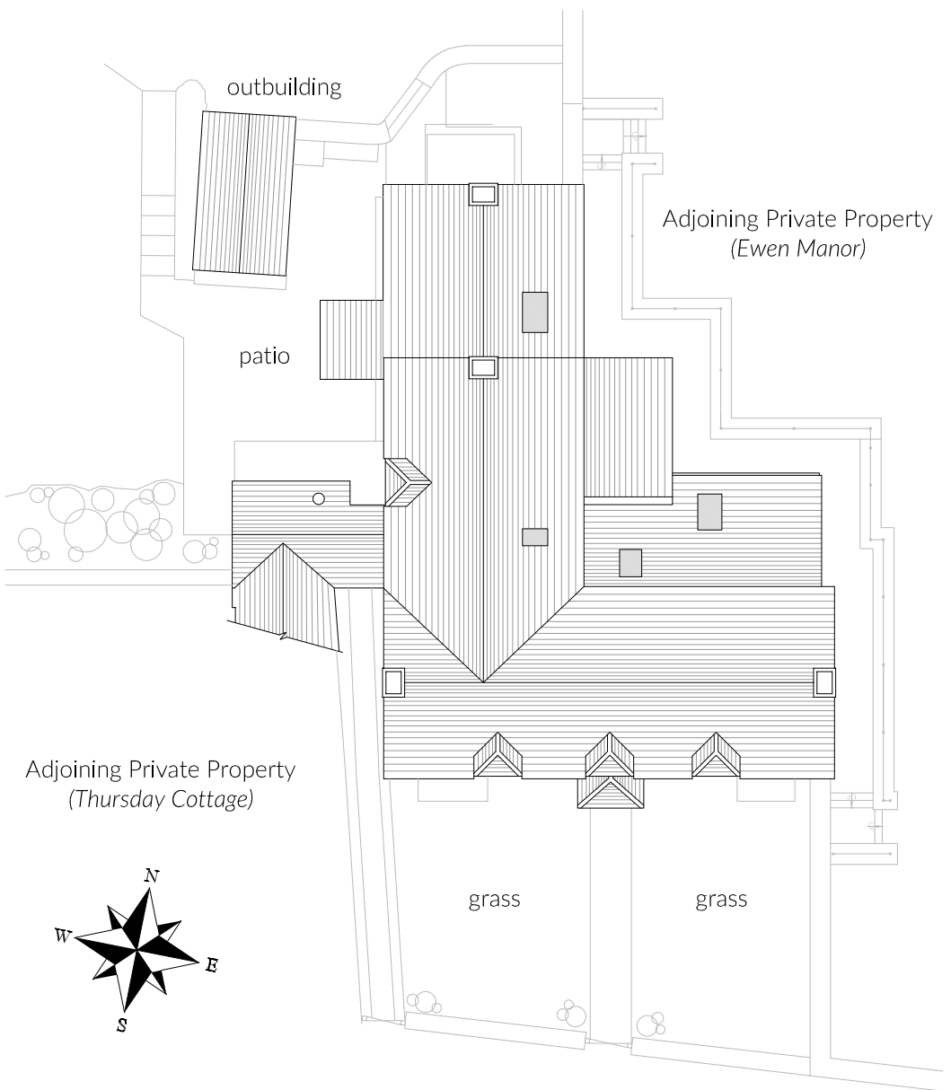
① Block Plan As Existing 1:200
