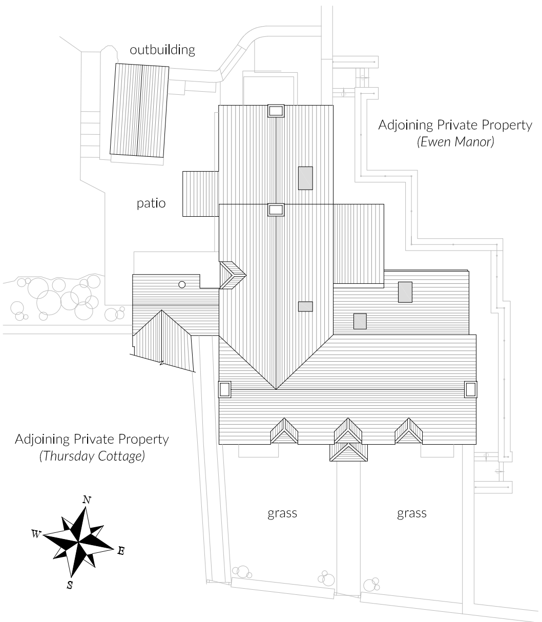
② Block Plan As Proposed 1:200
