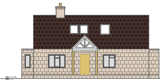
7 PORCH 1:100
