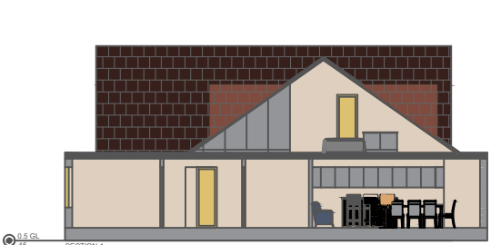
SECTION-1 1:100
