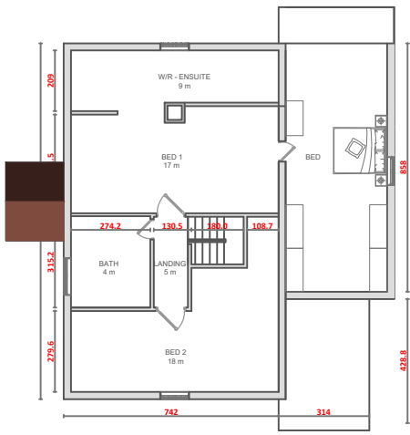
2 3 FF PROP PLANNING 1:100
