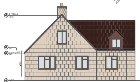
4 EX FRONT 1:100
