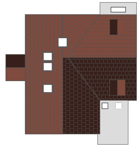
8 RIDGE PROP 1:100
