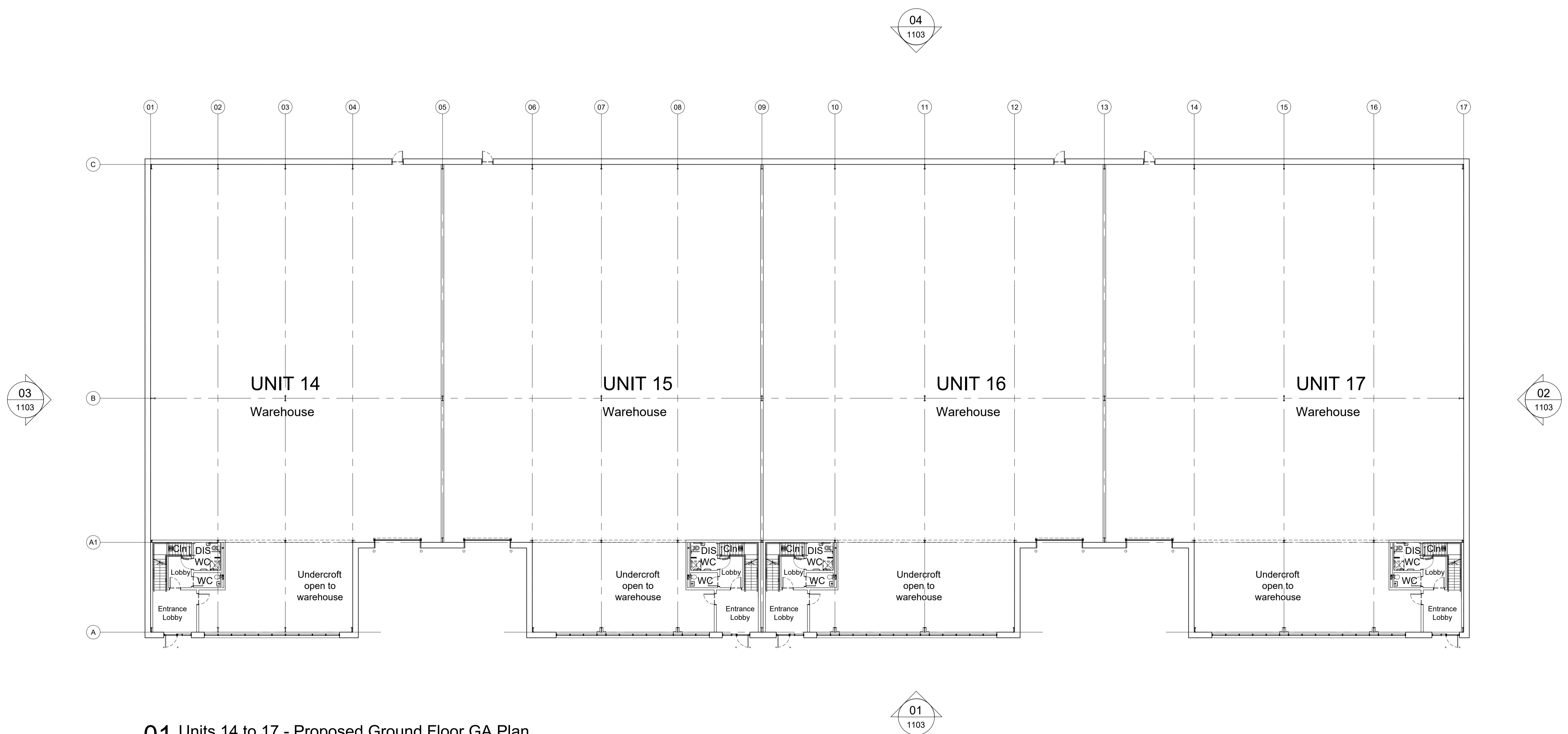
01 Units 14 to 17 - Proposed Ground Floor GA Plan 1:200 @ A1 / 1:400 @ A3
