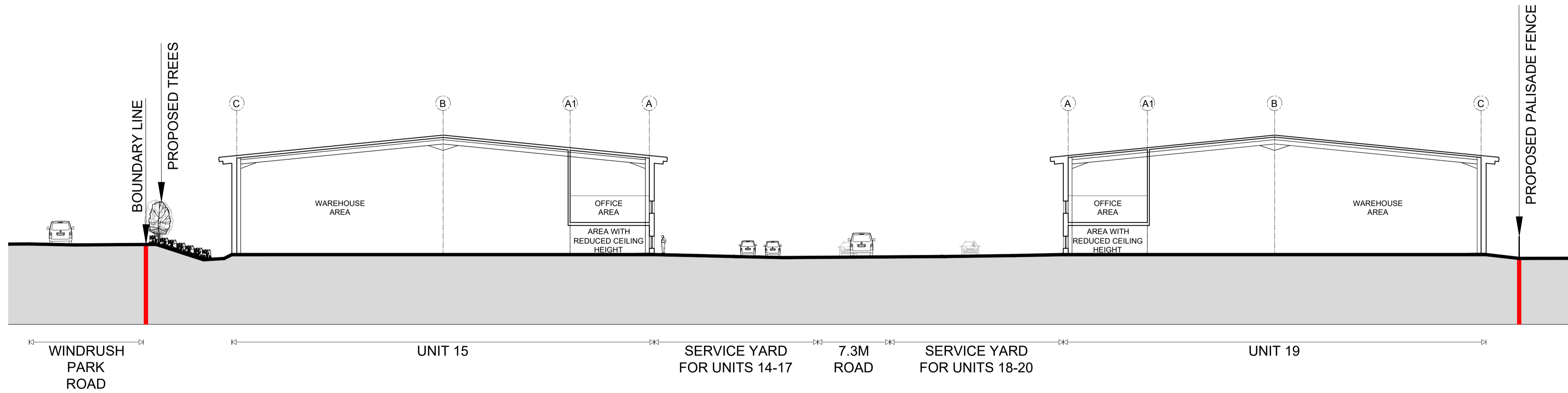
01 Proposed Site Section A'A through the site 1:250 @ A1 / 1:500 @ A3
