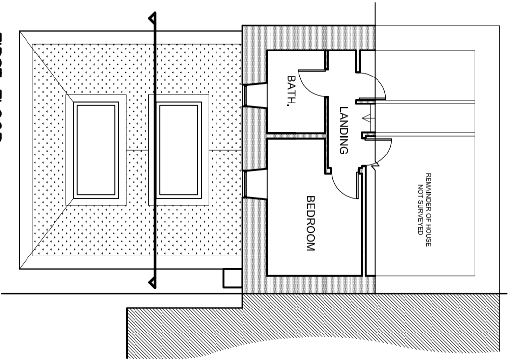
FIRST FLOOR
