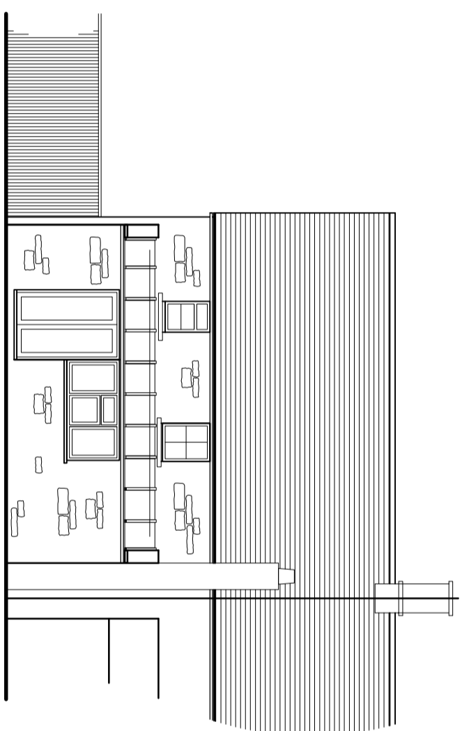
REAR ELEVATION
